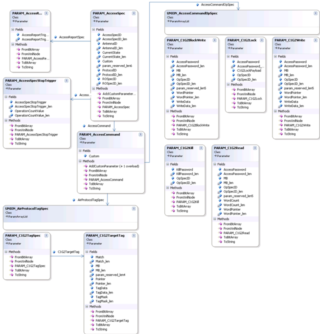
Figure 5.15 LTKNET – Core AccessSpec Classes
