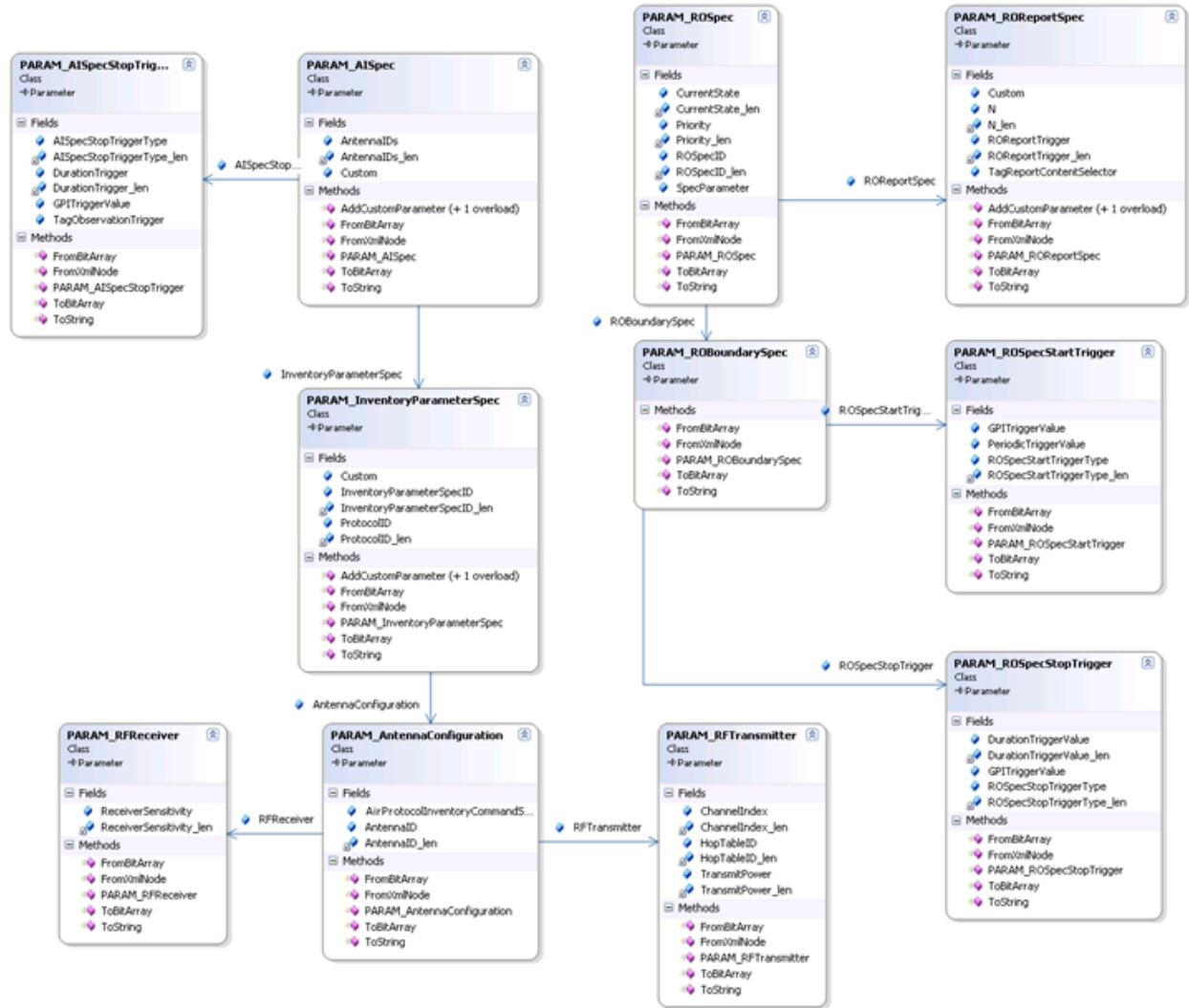
Figure 5.14 LTKNET – Core RoSpec Classes
