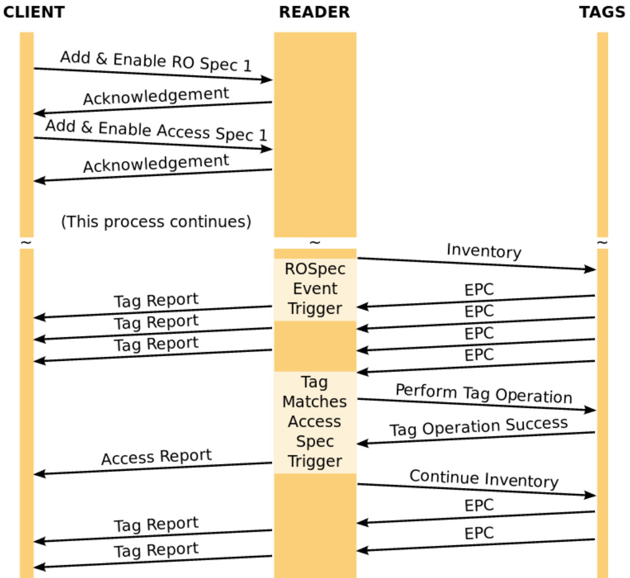
Figure 2.1 Sample LLRP Application Flow
