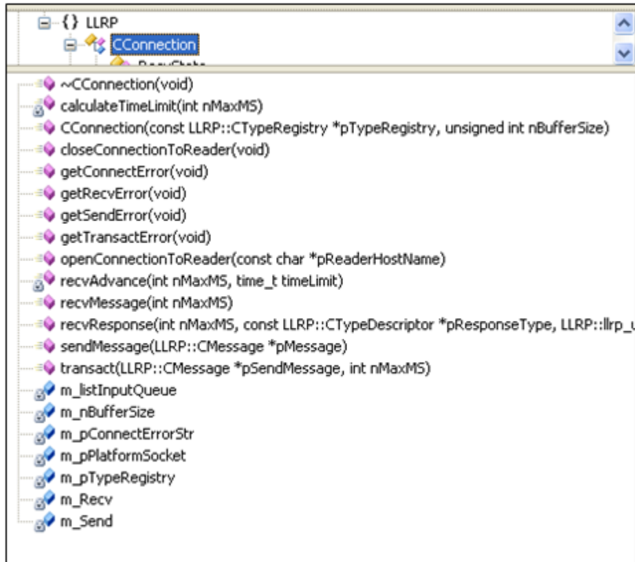
Figure 5.1 LTKCPP CConnection Class
